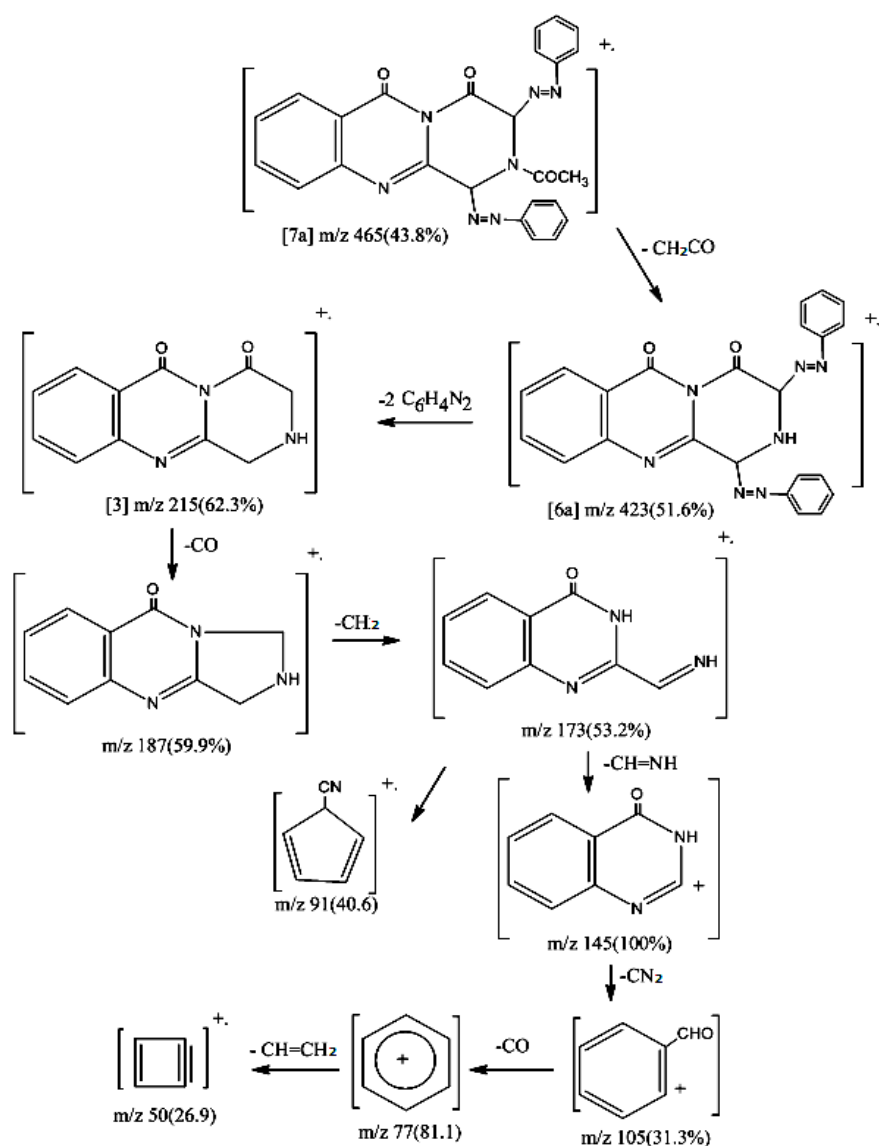
Scheme IV. Main fragmentation pathway of compounds [3], [6a] and [7a].
