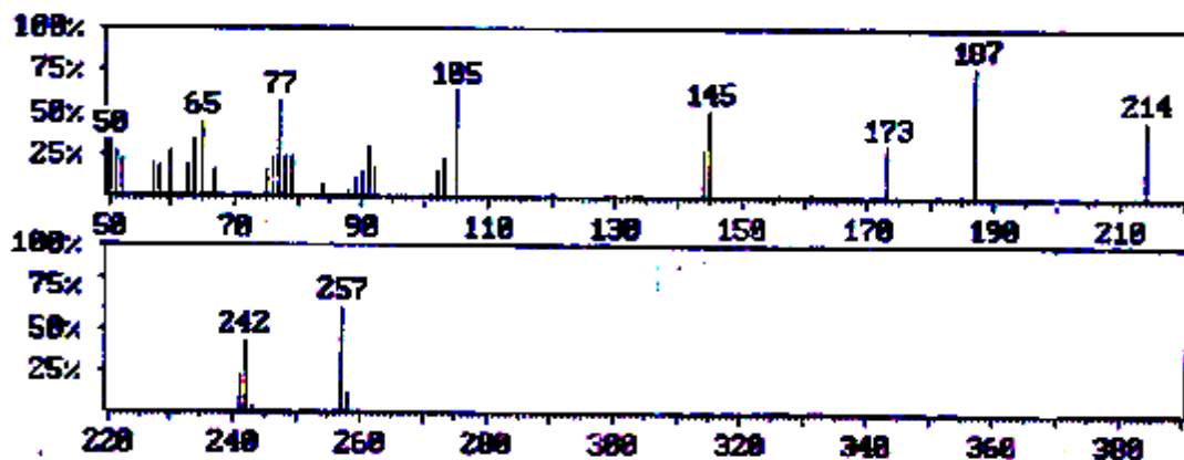
Fig.4 70 eV mass spectrum of compound [4]
