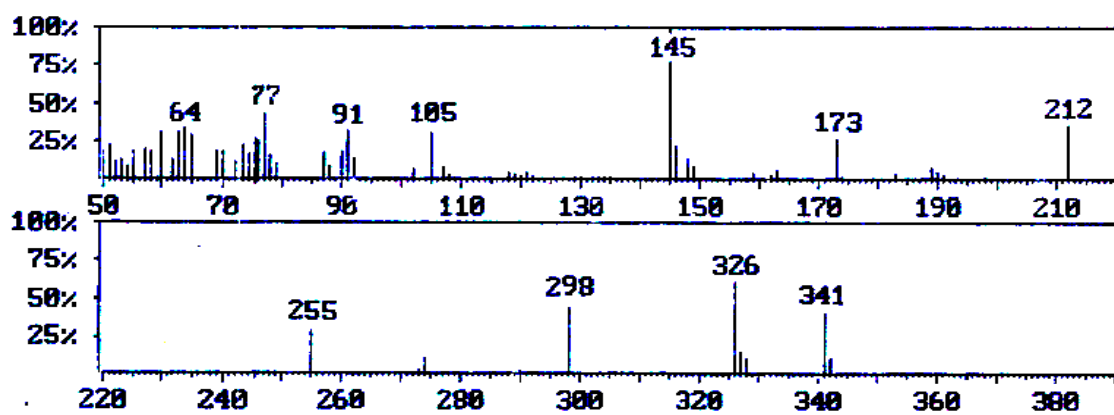
Fig.5 70 eV mass spectrum of compound [5]
