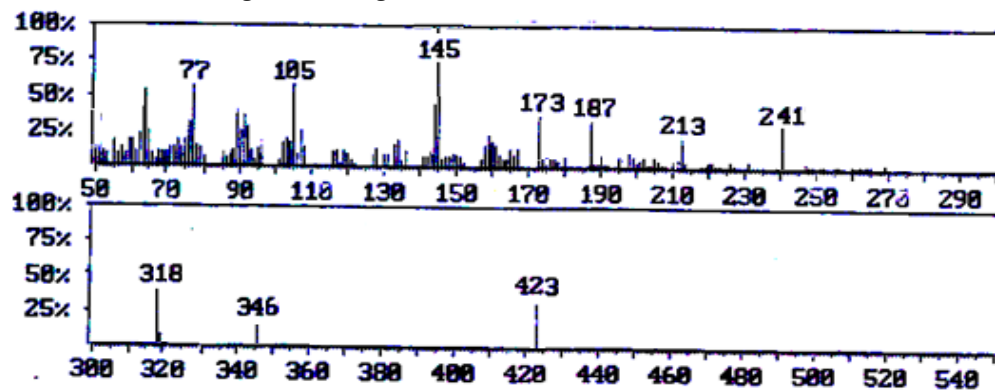
Fig.6 70 eV mass spectrum of compound [6a]
