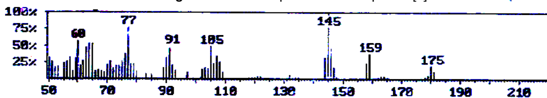
Fig.2 70 eV mass spectrum of compound [2]
