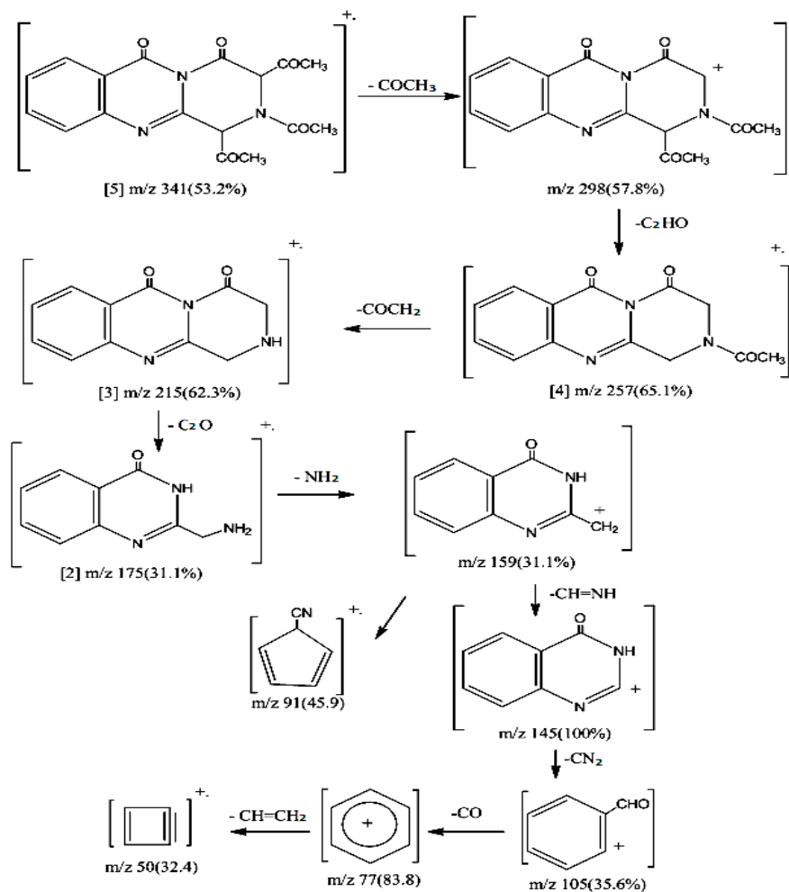
Scheme III. Main fragmentation pathway of compounds [2],[3],[4]and [5].
