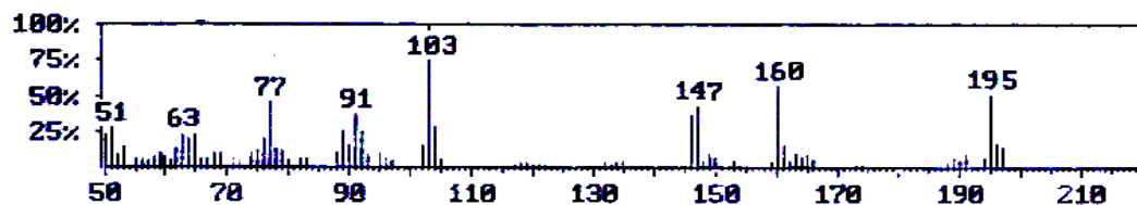
Fig.1 70 eV mass spectrum of compound [1]
