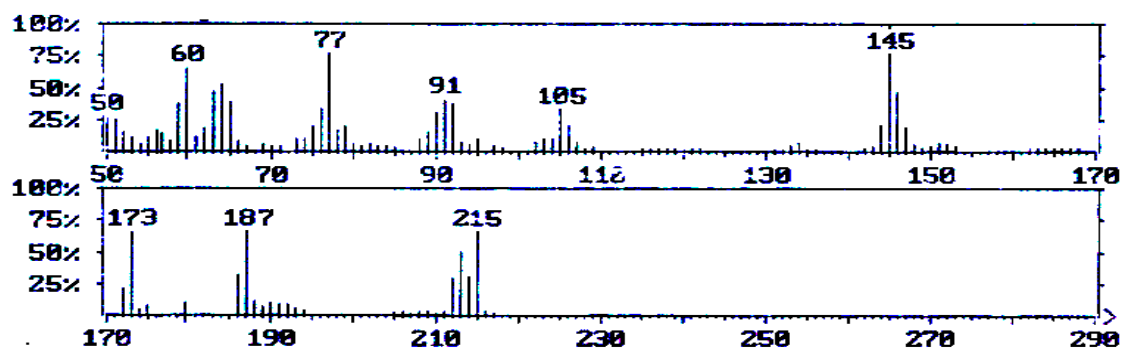
Fig.3 70 eV mass spectrum of compound [3]
