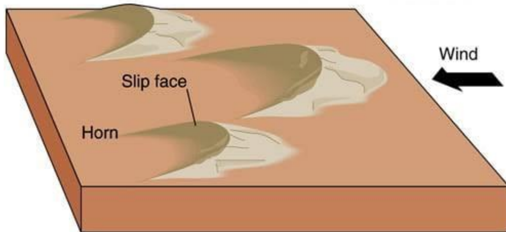
A Barchans
