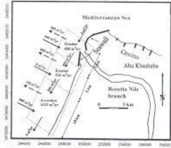
Figure 5. Sediment budgets calculated within the three sub-coastal stretches along the study area. Sediment volume is multiplied by 10^7 .
